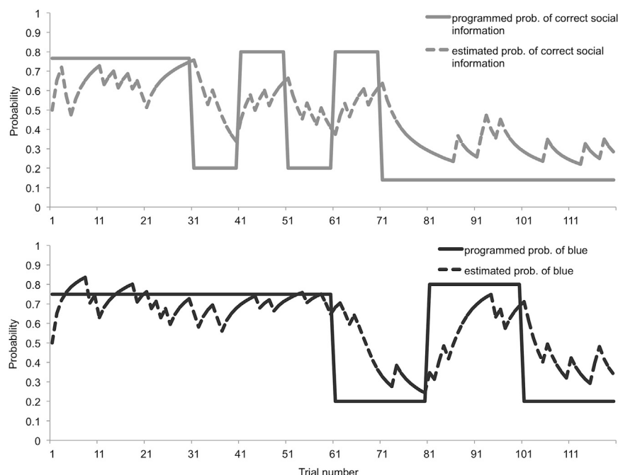
Figure 2. Social and Individual Bayesian Learner Models
